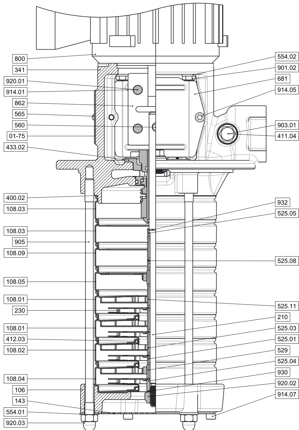
Figure 15: Sectional drawing DPVCI 2-10 B
