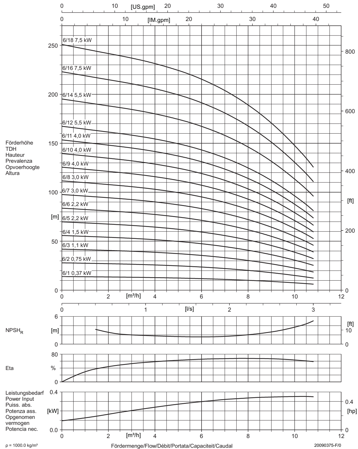
Figure 12: Performance curve DPVCI 6 B - 60Hz - 2 pole
