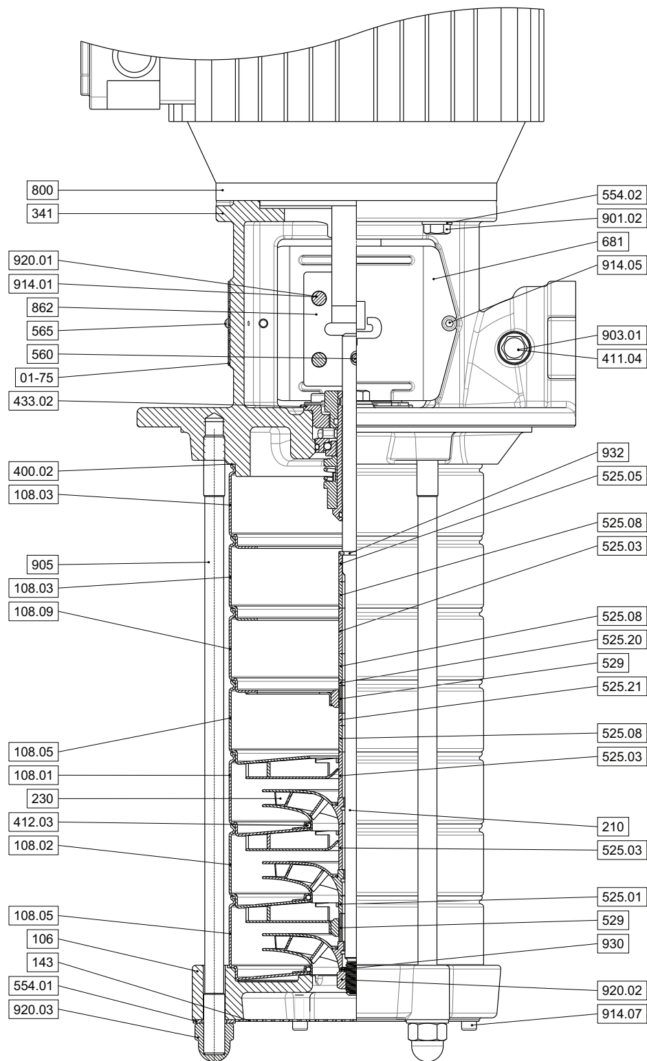
Figure 16: Sectional drawing DPVCI 15 C
