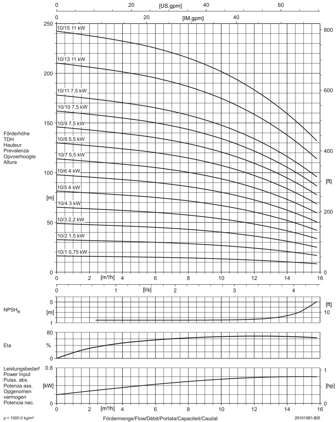
Figure 13: Performance curve DPVCI 10 B - 60Hz - 2 pole
