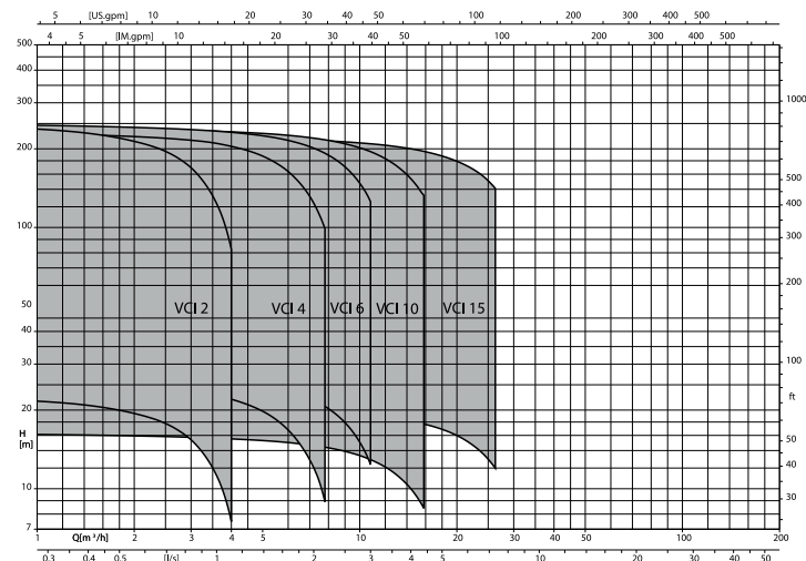
Figure 2: Performance range DPVCI 2, 4, 6, 10B, 15C 60Hz
