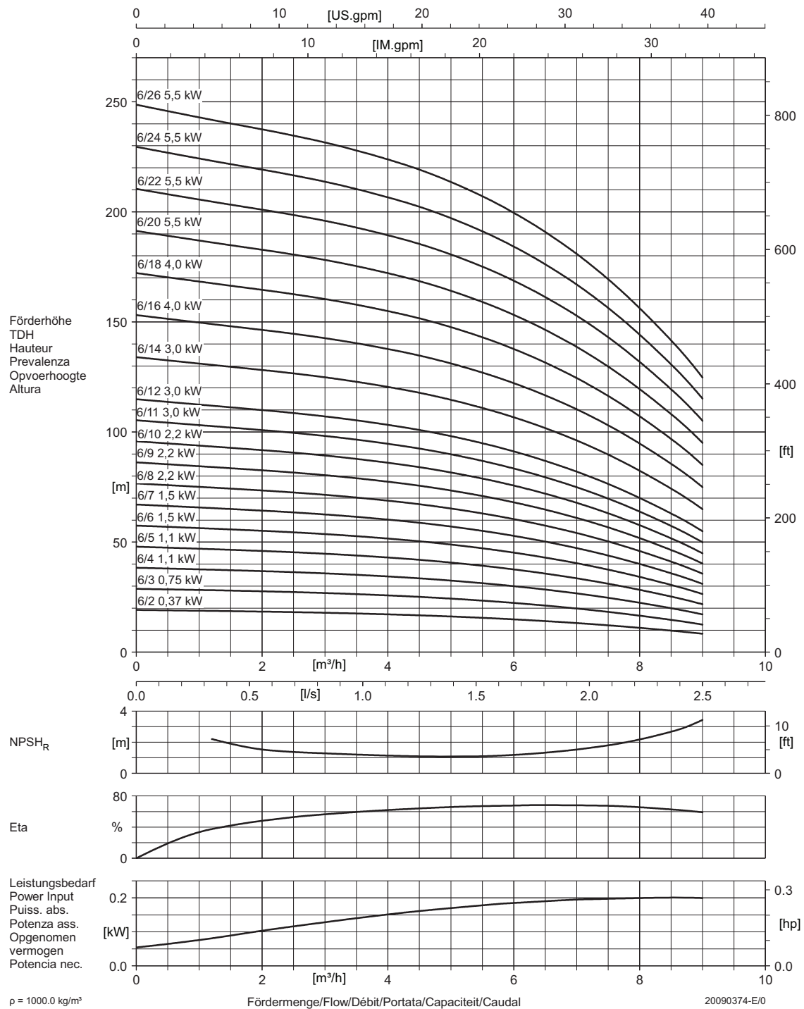
Figure 7: Performance curve DPVCI 6 B - 50Hz - 2 pole
