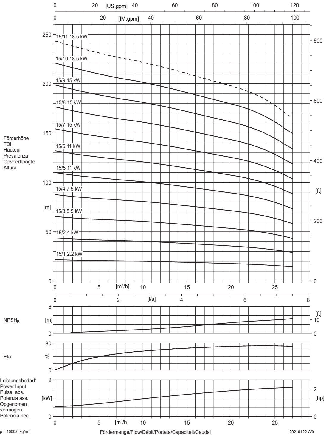
Figure 14: Performance curve DPVCI 15 C - 60Hz - 2 pole
