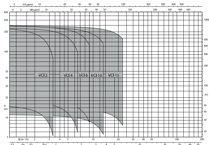
Figure 1: Performance range DPVCI 2, 4, 6, 10B, 15C 50Hz
