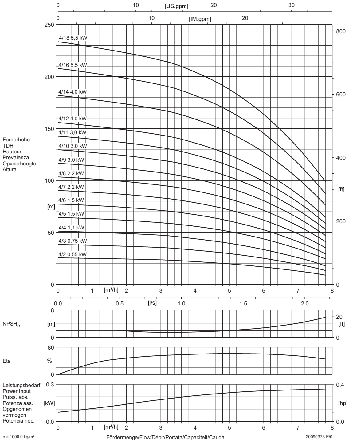
Figure 11: Performance curve DPVCI 4 B - 60Hz - 2 pole
