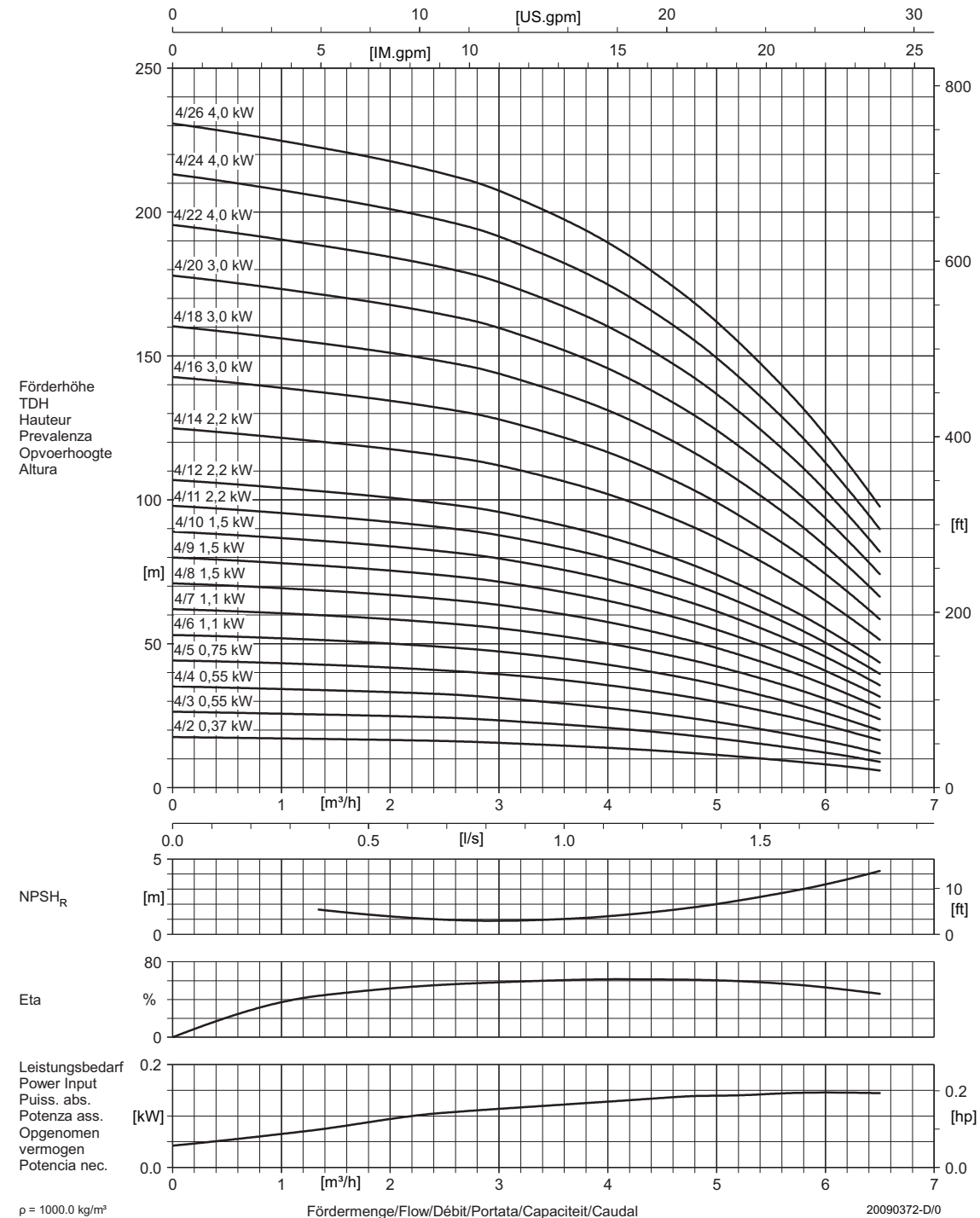
Figure 6: Performance curve DPVCI 4 B - 50Hz - 2 pole
