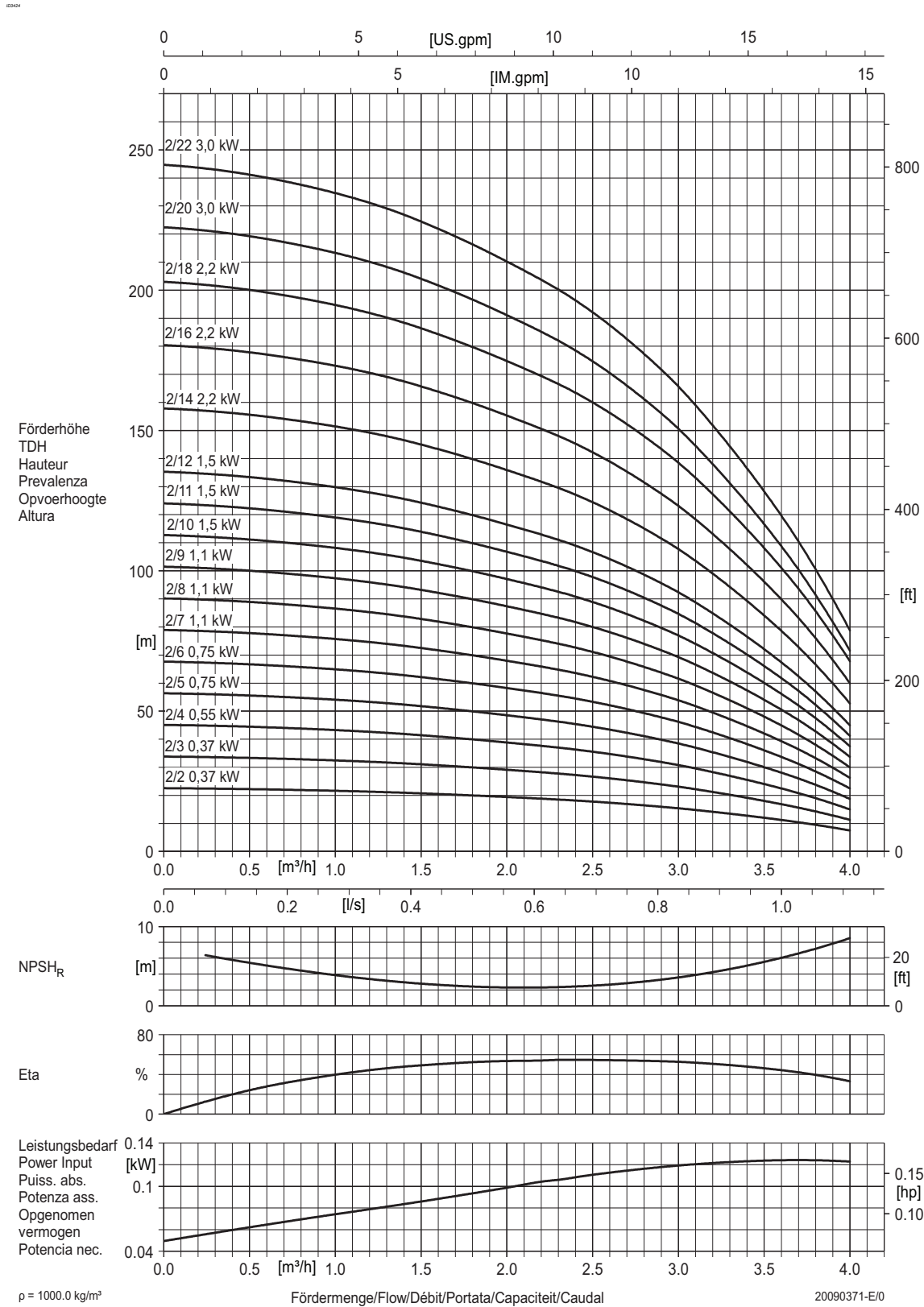
Figure 10: Performance curve DPVCI 2 B - 60Hz - 2 pole
