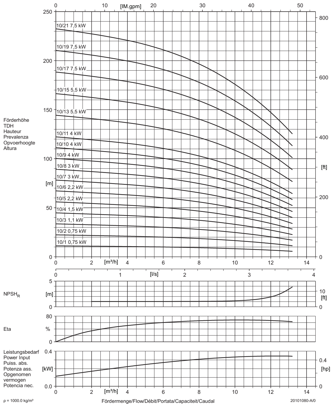
Figure 8: Performance curve DPVCI 10 B - 50Hz- 2 pole
