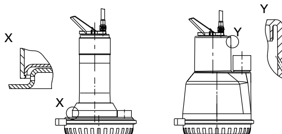
Afb. 5: Ontluchtingsopening
